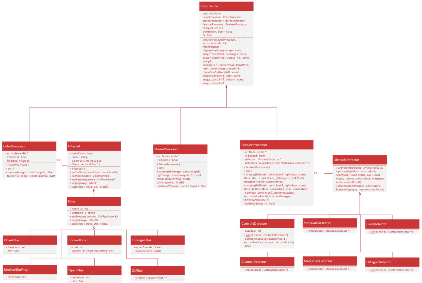
Vision UML
